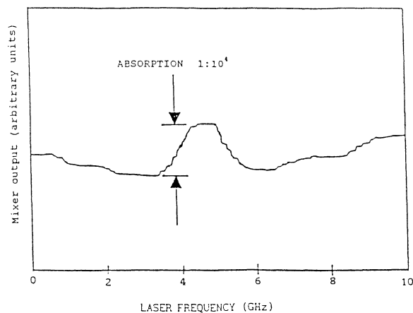
Fig. 17. FM spectroscopy signal from a sample of atomic sodium exhibiting a 0.01 percent absorption.
