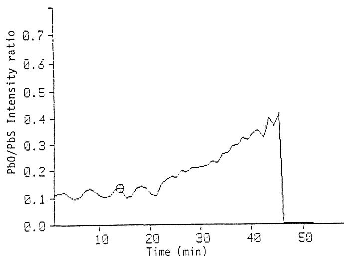
Fig. 1. Time behaviour of the PbO/PbS intensity ratio close to the end of a slag blow.
