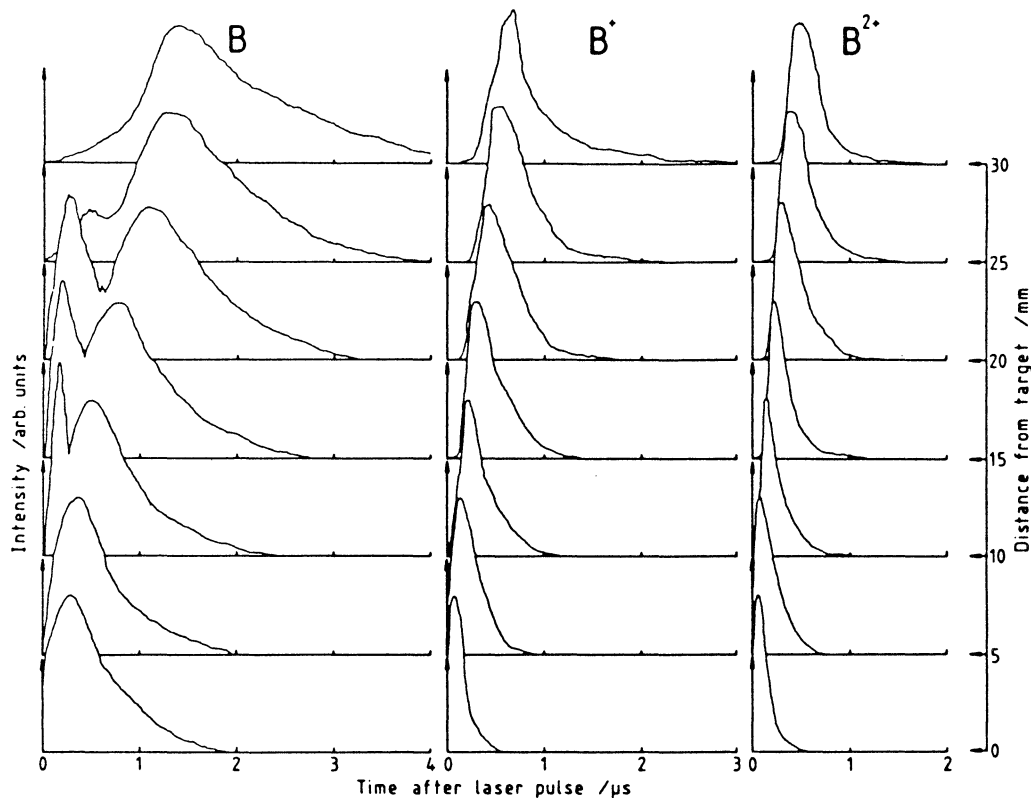
Fig. 12. Diagram showing the propagation of B , B^+ and B^{2+} in an expanding boron plasma. The detected transitions are, in B : 3s\ ^2S-2p\ ^2P at 249.7 nm, in B^+ : 4f\ ^1F-3d\ ^1D at 494.0 nm and in B^{2+} : 5g\ ^2G-4f\ ^2F at 449.9 nm. The intensities of the pulses are normalized to one.
