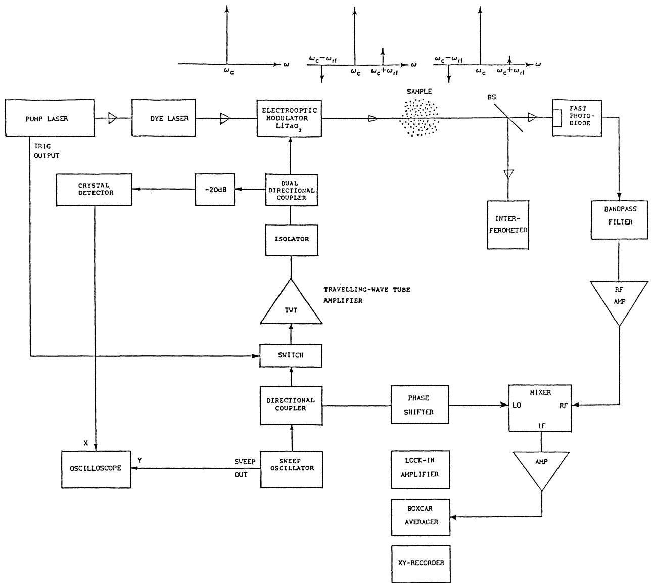
Fig. 16. Experimental arrangement for FM spectroscopy using microwaves.
