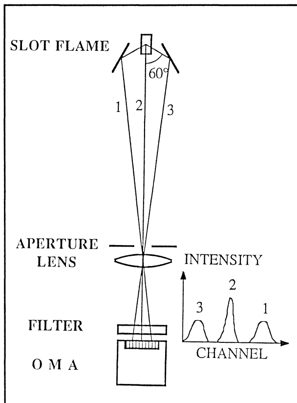
Fig. 8. Experimental arrangement for simultaneous recording of 3 emission projections.
