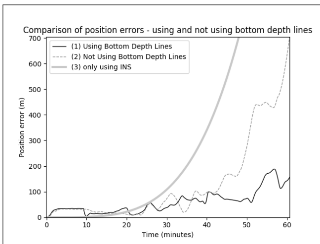
Figure 35: Test 6:2: The medium-accuracy INS is used. It shows a good performance during 45min, even though the bottom depth lines are not being used. After this time, it has problem tracking the correct position.
