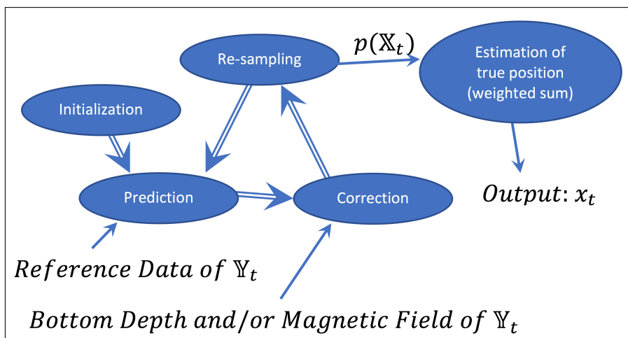
Figure 22: A block diagram of the Particle Filter used in our implementation. After initialization, the particle filter iterates between Prediction , Correction and Re-sampling . After the Re-sampling Step , a probability of each state p(\mathbb{X}_t) is estimated from the particles. From this, a weighted sum of all particles can be used as an estimation of the true position.
