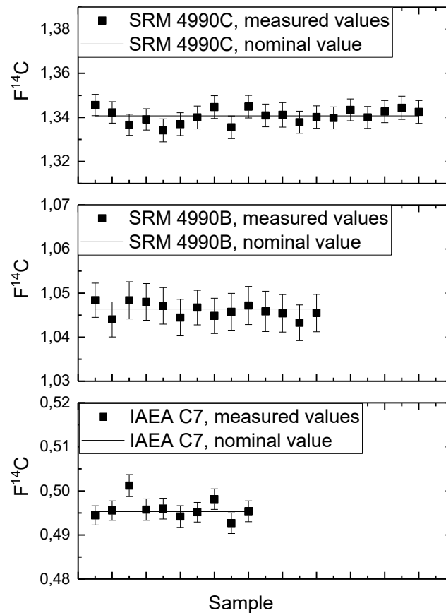
Figure 15. Results of the ^{14}\text{C} measurements of standard samples IAEA C7, SRM 4990B (also known as OxI) and SRM 4990C (also known as OxII). Uncertainty bars refer to 1\sigma .
