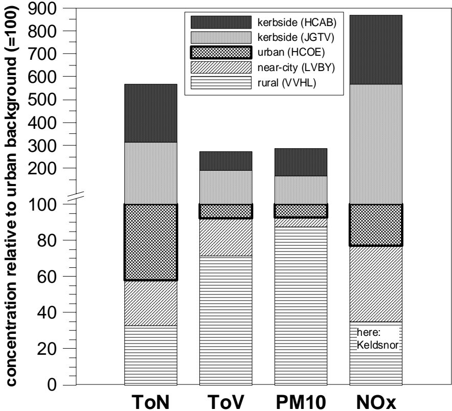
Figure 20: Comparison of average concentrations of total particle number (ToN), total particle volume (ToV), PM10 and NOx at rural (VVHL=Vavibill), near-city (outside Copenhagen) urban and kerbside stations relative to urban background levels (in Copenhagen). The concentration levels are cumulative so that only the difference between the level below appears as a specific pattern. The elevation of the urban background (HCOE) above the near-city level is shown by bold lines and represents the potential for urban emission reduction measures to decrease urban concentrations. Note that the scale of the vertical axis changes at 100. Since NOx was not measured at Vavibill, data from another rural station (Keldsnor) was used to represent background contributions (from Paper IV).
