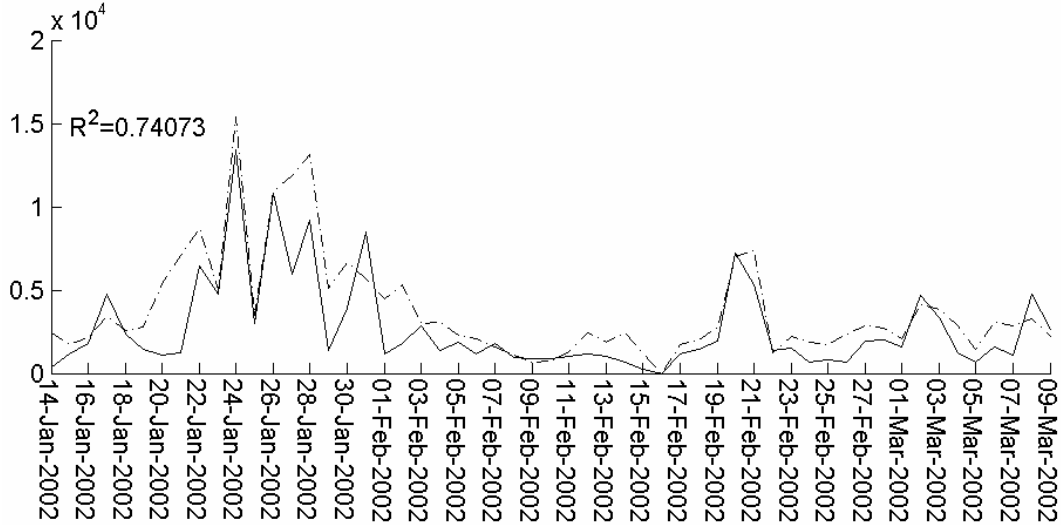
Figure 15: Daily average contribution to the particle number concentration ( cm^3 ) from both domestic wood combustion and long range transport during the entire measurement period in Forsdala, Lycksele. Source/receptor modelling results are shown with the continuous line and dispersion modelling results with a dashed-dotted line. The coefficient of determination ( R^2 ) between the two modelling runs is given in the Figure (From Paper III).
