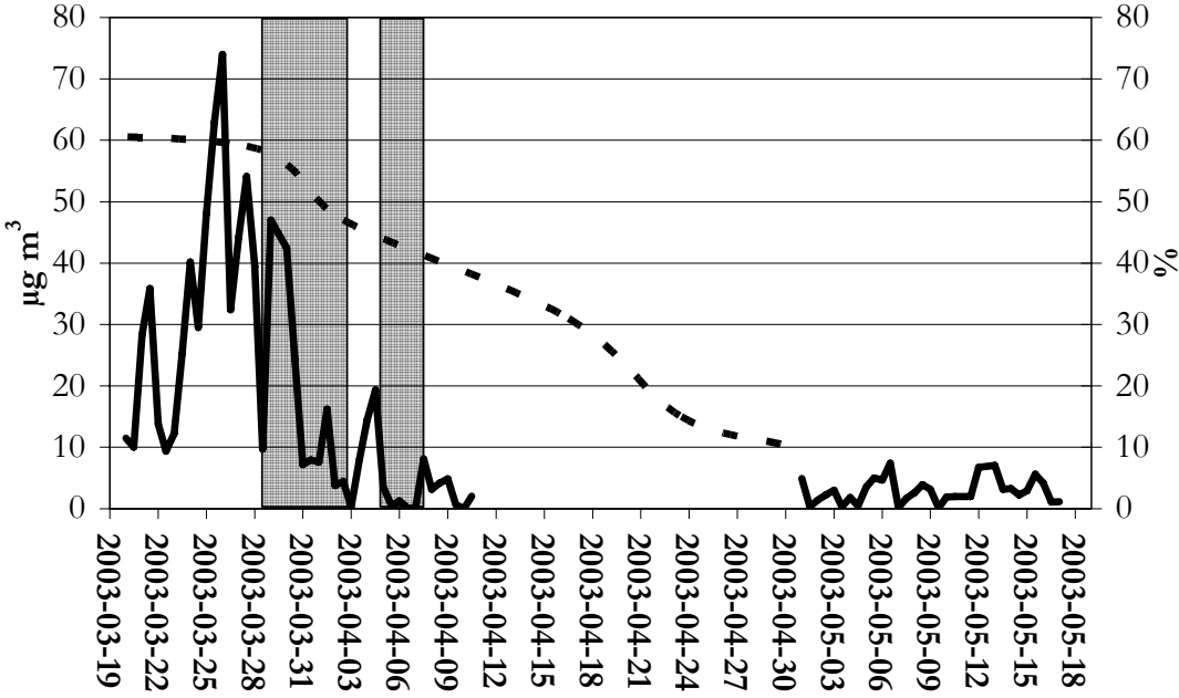
Figure 16: The fraction of cars using studded tyres (dashed line) and the re-suspended fraction of PM10 (continuous line) (from Johansson et al., 2005). The grey shaded areas show periods of rain.
