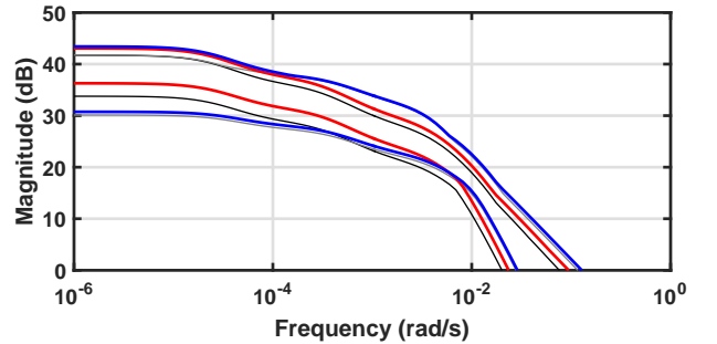
Fig. 2. Bode diagram of allometrically scaled pediatric model set, linearized for induction of anesthesia, compared to the set scaled by body weight. The minimal and maximal Bode magnitude of the set scaled with w_{alo} is shown for patients aged 6-10 in red, and patients aged 11-16 in blue. The minimal and maximal magnitudes for the model set scaled with body weight are shown in black (aged 6-10) and grey (aged 11-16).
