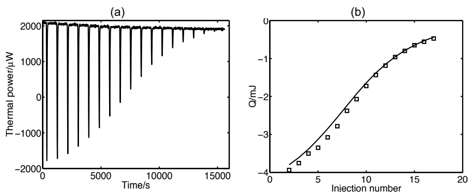
Figure 5.7 (a) Thermal power as a function of time for sequential 4.16 \mu\text{L} injections of 0.1116 \text{ mol kg}^{-1} B_{12} into 4.746 \text{ mmol kg}^{-1} \beta -CD aqueous solution at 308.20 K. (b) Heat ( Q ) per injection versus injection number at 308.20 K, ( \square ) are experimental points and (—) fitted line.
