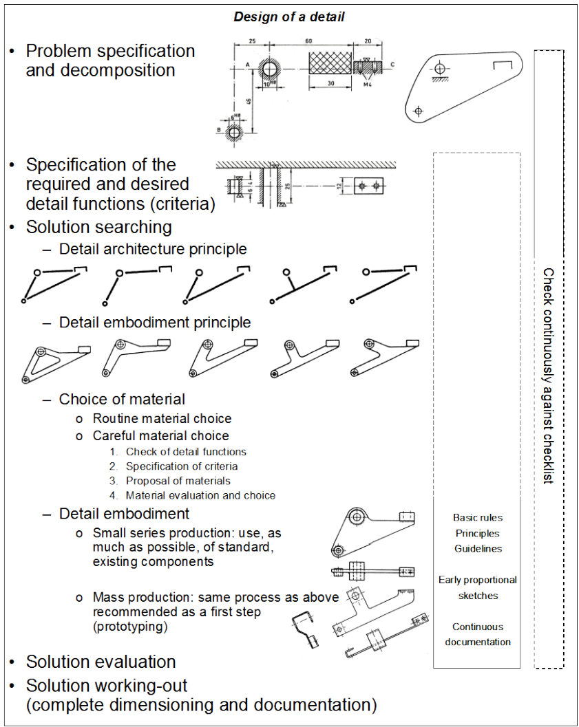
Figure 1. Model for embodiment design and detail design process.
