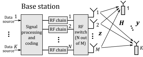
Fig. 5. System model of a multi-user MIMO system with transmit antenna selection.
