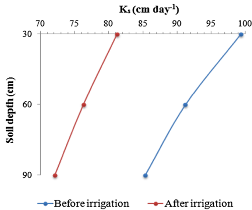
Fig. 6 Measured saturated soil hydraulic conductivity ( K_s ) values before and after irrigation at different soil depths
