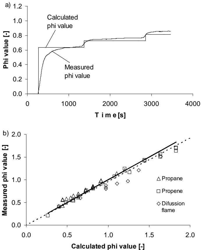
Figure 12. a) Measured and calculated phi values from an experiment on the combustion of propane, as a function of time.
