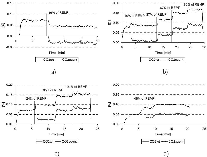
Figure 19. Production of CO 2 as a function of time, a) test 2 with Halon 1301, b) test 1 with HFC 125, c) test 2 with HFC227ea, d) test 3 with C 6 F-ketone.
