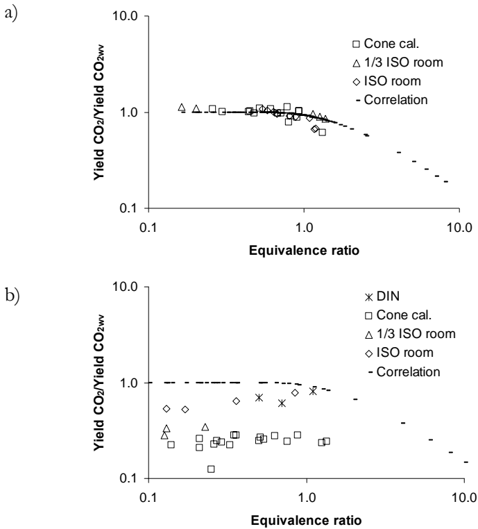
Figure 17. a) Ratio of the yield of CO 2 to the maximum yield of CO 2 for well-ventilated conditions in experiments with Nylon 6,6. The dashed line shows the Tewarson correlation.
