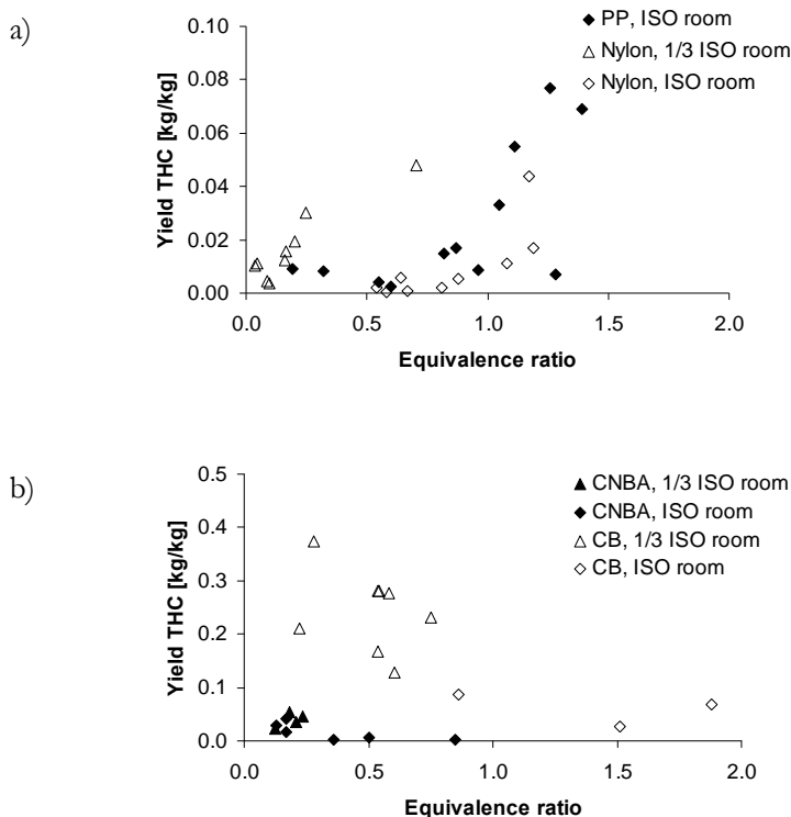
Figure 21. a) The yield of unburned low-molecular-weight hydrocarbons is presented as a function of the equivalence ratio for experiments with PP and Nylon 6,6.
