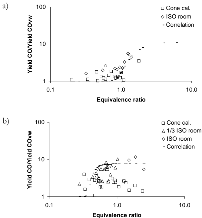
Figure 18. a) Ratio of the yield of CO to the CO yield for well-ventilated conditions during experiments with PP. The dashed line shows the Tewarson correlation. b) Ratio of the yield of CO to the CO yield for well-ventilated conditions during experiments with CB. The dashed line shows the Tewarson correlation.
