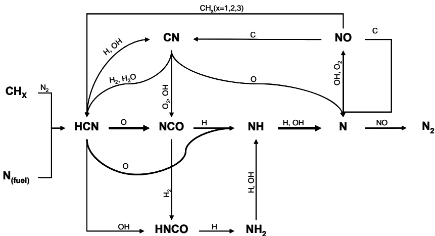
Figure 31. Reaction scheme for the transformation of fuel-bound-nitrogen to NO x and HCN [70].
