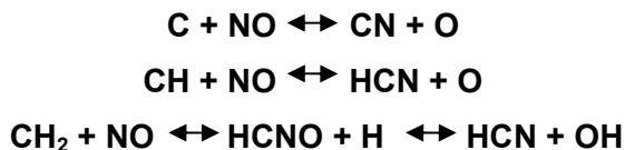
Figure 32. Possible reactions for production of nitrogen oxides in the presence of hydrocarbons [73].
