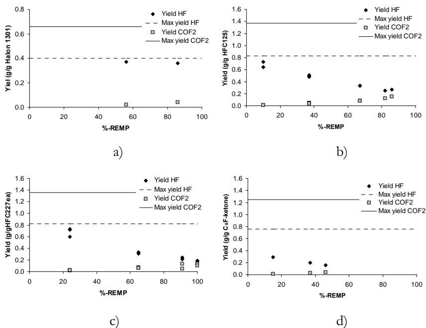
Figure 38. Yields of halogen containing combustion products from the tests with: a) Halon 1301, b) HFC 125, c) HFC 227ea and d) C 6 F 12 O-ketone.
