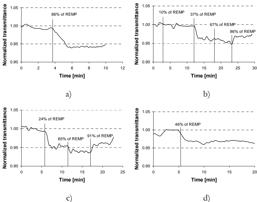
Figure 24. Normalised transmittance of the combustion gases as a function of time, a) test 2 with Halon 1301, b) test 1 with HFC 125, c) test 2 with HFC 227 ea, d) test 3 with C 6 F-ketone.
