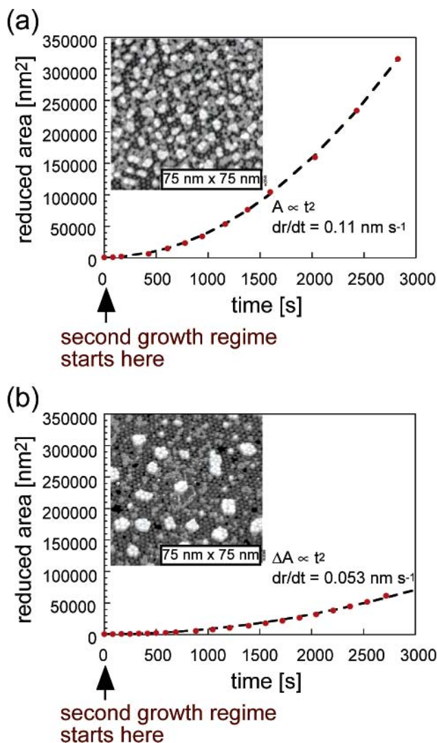
Figure 7. Growth of a single reduced patch at 1 \times 10^{-7} mbar H 2 for (a) the normal preparation of the oxide and (b) a smoother surface oxide created by removal of 0.21 ML before oxidation. Surface b has fewer domain boundaries, fewer islands, but slightly more holes (inset).
