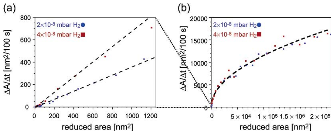
Figure 6. Comparison of the reduction speed over time for 2 \times 10^{-8} mbar H 2 and 4 \times 10^{-8} mbar H 2 . (a) Initial reduction speed (first growth regime, linear fit) that scales with the pressure. (b) Reduction speed for large reduced areas (second growth regime, square root fit) that is pressure-independent.
