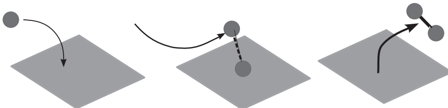
Figure 5.3: Eley-Rideal mechanism model.
