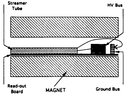
Fig. 2: Access to the cathode of the streamer tube
