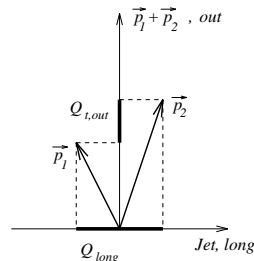
Figure 1: LCMS projection on the (Q_{long}, Q_{t,out}) plane.
