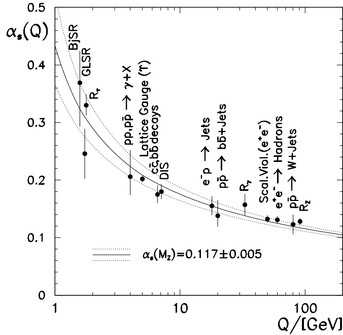
Figure 3.2: Different \alpha_s measurements compared to the QCD prediction based on the averaged value of \alpha_s(M_Z) = 0.117 \pm 0.005 .
