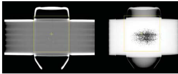
Figure 2. kV images of the phantom taken with the OBI at 0° (left) and 270° (right). The images were matched against the DRR generated in the TPS and used to correct for the offset.
