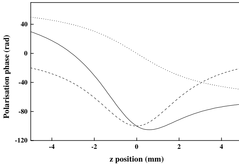
Figure 3.5 The phase of the polarisation along the propagation axis (solid line). The phase due to the focusing is shown with a dotted line and the intensity dependent phase is shown with a dashed line.
