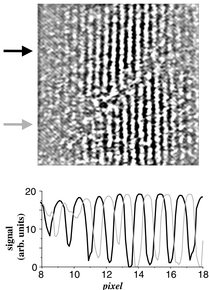
Figure 5.7 Interference pattern obtained with the 13 th harmonic probing an aluminium step filter together with a cross-section of the contrast above (black) and below (grey) the transition region.
