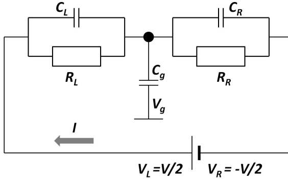
Figure 2.1: A single-electron transistor represented as an element of a dc-circuit. The left and right junctions are described by their capacitance and resistance, respectively. Gate capacitance and gate voltage control the island energy landscape.
