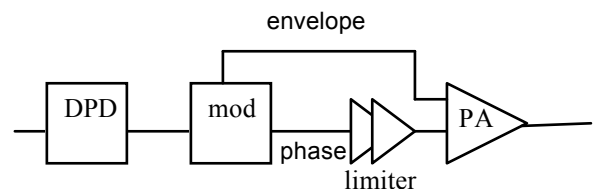
Fig. 1. Transmitter architecture.
