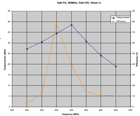
Fig. 4. Simulation results for V_{dd} = 18 V, V_{in,peak} = 10 V and V_{bias} = -3 V.
