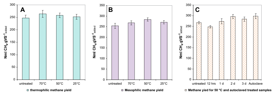
Fig. 3. (A) Normalised methane yields (Nml \text{CH}_4 \text{gVS}_{\text{added}}^{-1} ) after thermophilic; (B) mesophilic anaerobic digestion of pre-treated sludge; (C) methane yield for 50 °C pre-treated sample.
