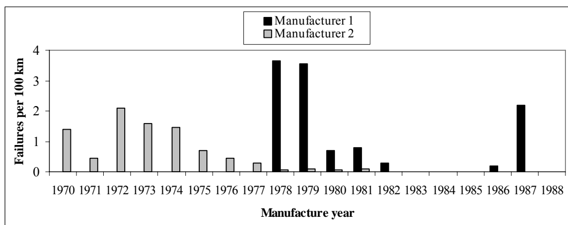
Figure 5, Manufacture year dependence: XLPE failure rate per 100 km cable, two different manufacturers, Manufacturer 1 data 1978-1988, Manufacturer 2 data 1970-1981
