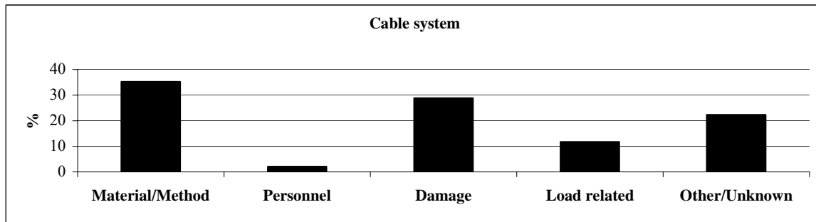
Figure 2, Failure statistics of cable systems 2005 [18]
