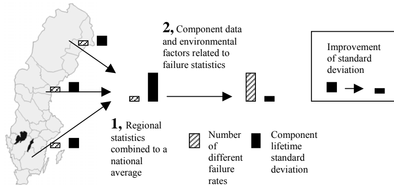
Figure 7, Schematic picture of national overhead line system failure statistics: National co-operation and failure statistics related to component data do not, to the same extent as in the case of cable systems, improve the standard deviation of estimated lifetime of overhead lines
