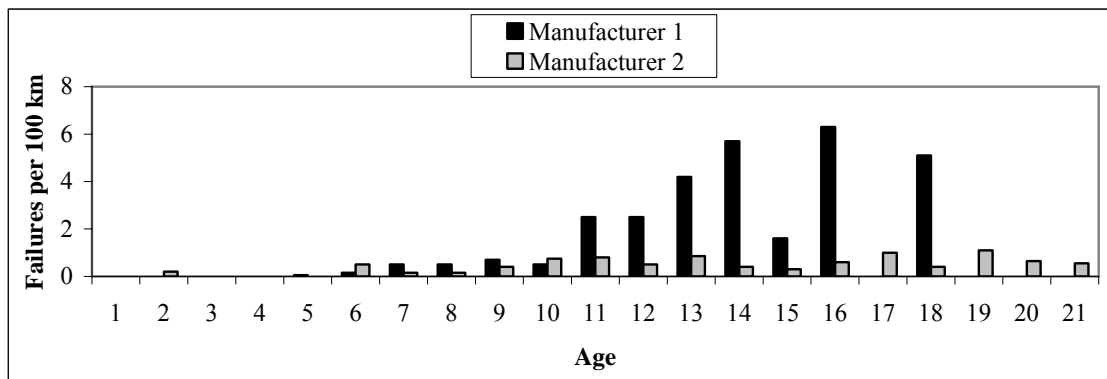
Figure 4, Component age dependence: XLPE failure rate per 100 km cable, two different manufacturers
