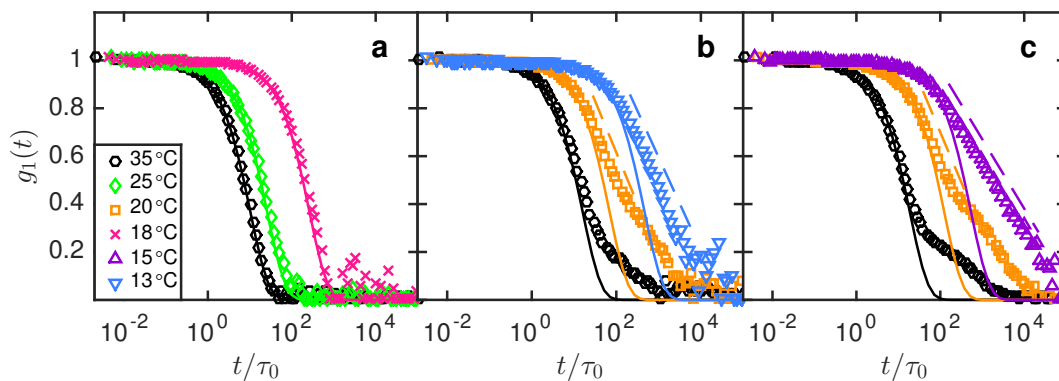
Figure 4.9: ISFs of \gamma B -crystallin in D_2O from DLS at \phi = 0.16 (a), 0.27 (b) and 0.33 (c). Also shown are exponential (—) and logarithmic fits (---, offset from the actual data for clarity).
