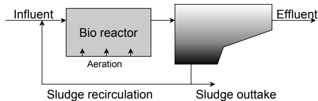
Figure 2.2 Simple activated sludge system
