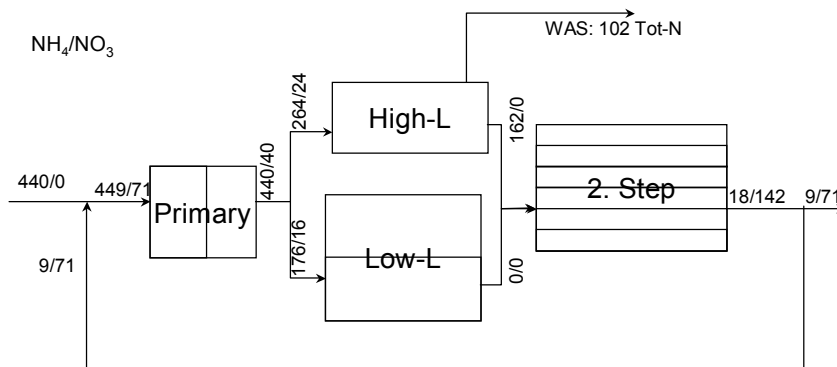
Figure 5.3 Nitrogen removal in the Lindau wastewater treatment plant according to Wilderer and Genes (1998). The first number denotes ammonium load, the second denotes nitrate load. The numbers are in kgN/day.
