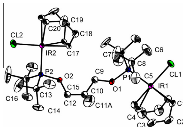
Fig. 2. DIAMOND drawing of compound 3 at the 30% probability level. Hydrogen atoms are omitted for clarity. Selected bond lengths ( \text{\AA} ) and angles ( ^\circ ) with estimated standard deviation: Ir1–C1 2.199(5), Ir1–C4 2.114(6), Ir1–P1 2.337(2), Ir1–C11 2.354(2), C11–Ir1–P1 95.44(7), C1–Ir1–C4 79.8(2).
