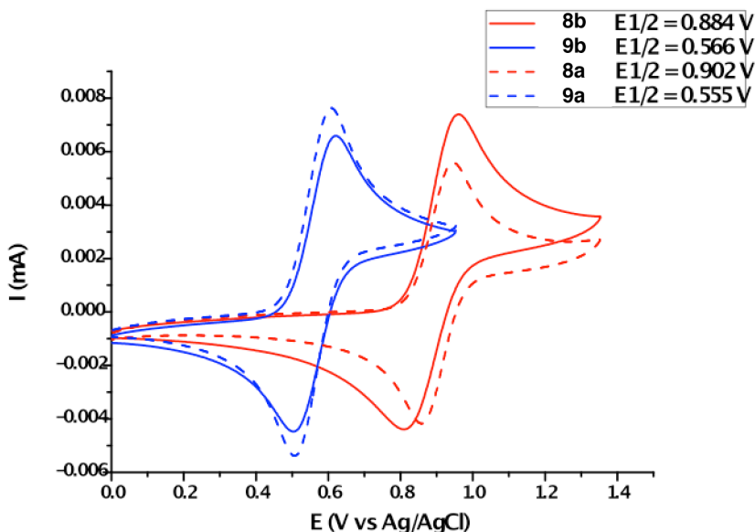
Figure 3.3. Cyclic voltammety scans of 10^{-3} M solutions of compounds 8-9 at a Pt electrode in \text{CH}_2\text{Cl}_2 (0.1 M (^t\text{Bu}_4\text{N})\text{PF}_6 scan rate 0.1 \text{ V s}^{-1} ).
