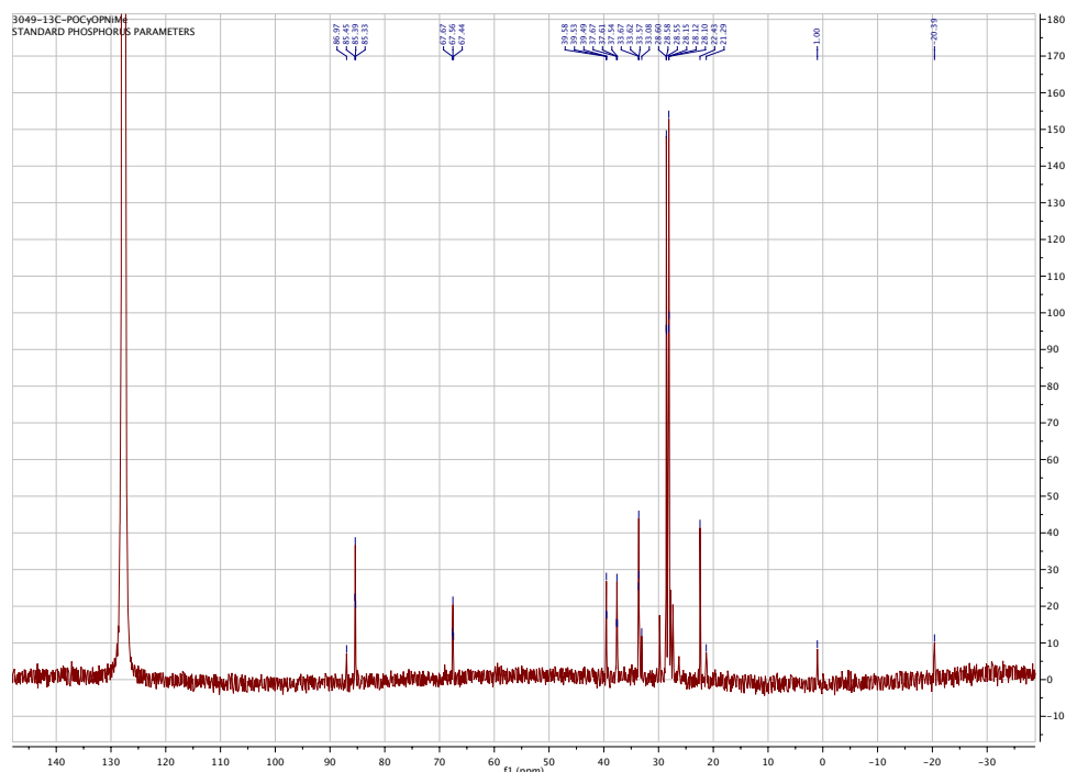
^{13}\text{C} -NMR ( \text{C}_6\text{D}_6 ) of compound 3. The Ni-Me carbon are displayed as a triplet at -20 ppm. Trace amounts of 1a are notable, especially for its more intense shifts i.e. the \text{CH}_2\text{CHO} carbons at 87 ppm, the \text{C}(\text{CH}_3)_3 carbons around 28 ppm and the \text{CH}_2\text{CH}_2\text{CH}_2 carbon at 21 ppm. The singlet at 30 ppm corresponds to Apiezon brand H grease, and the singlet at 1 ppm is silicon grease.
