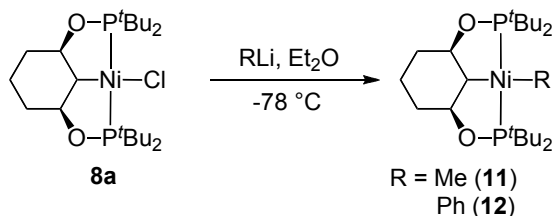
Scheme 3.8. Synthesis of compounds 11 and 12 .
