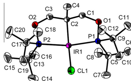
Fig. 1. DIAMOND [18] drawing of compound 2 at the 30% probability level. Hydrogen atoms and solvent benzene are omitted for clarity. Selected bond lengths ( \text{\AA} ) and angles ( ^\circ ) with estimated standard deviation: Ir1–C2 2.108(3), Ir1–C11 2.413(1), Ir1–P1 2.2916(8), Ir1–P2 2.2844(9), P1–Ir1–P2 162.65(3).
