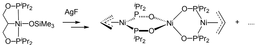
Scheme 2.8. Zargarian's isolated decomposition products from attempted formation of a \text{POC}_{\text{sp}^3}\text{OP} nickel fluoride complex.
