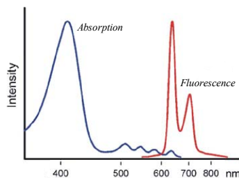
Figure 5.5. The absorption and emission spectrum of PpIX.
