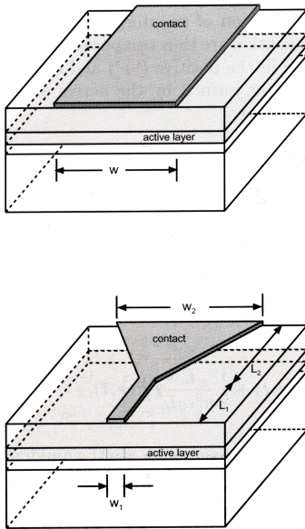
Figure 2.15. On top the broad area laser geometry, featuring a very wide stripe width. Below the tapered device, showing the single-moded structure and the tapered amplifier.
