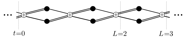
Fig. 6: The convolutional protograph of Example 3, along with some termination factors for increasing L .
