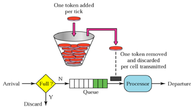
Figure 3. Token bucket [Forouzan 2004]
