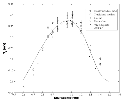
Figure 6 The measured and computed flame speeds for methane at T_u=25 °C.
