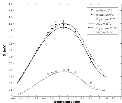
Figure 7 The measured and computed flame speeds for methane at T_u=25 °C and T_u=270 °C.
