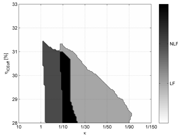
Figure 4.16 Optimal combinations of controller parameters for linear feedback term and nonlinear feedback term. The abbreviations have the following meaning: L inear F eedback, N on L inear F eedback.
