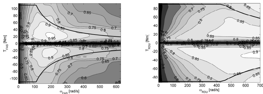
Figure 3.3 Electrical machine efficiency for the FAS (left) and RDU (right).
