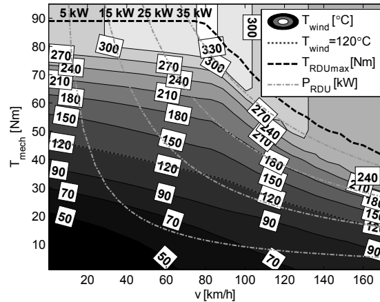
Figure 8.5 Winding end temperature as a function of torque and vehicle speed. Temperature of the cooling liquid and DC-voltage are equal to 25 °C and 300 V, respectively.
