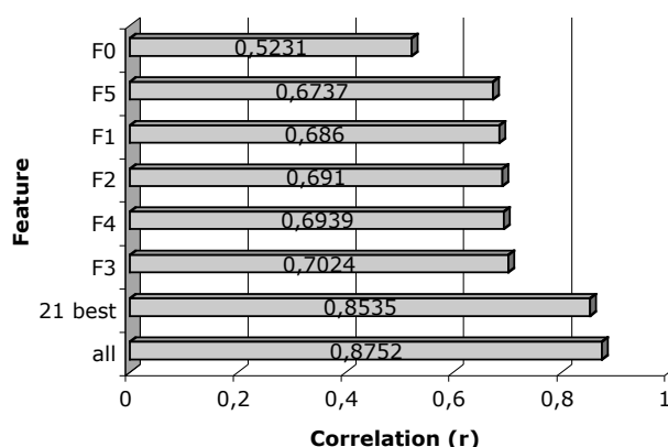
Figure 2. Correlations between chronological and estimated age for the best feature CARTs.
