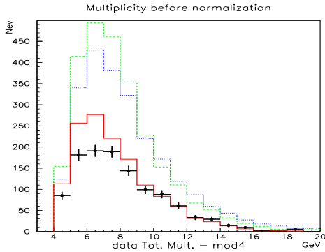
Figure 7.3: The multiplicity distribution of single tag events measured by module 4 of VSAT in year 2000 before normalization. The points are data, TWOGAM is shown as a solid line, PHOJET as a dashed line and PYTHIA as a dotted line.
