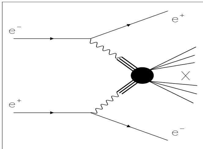
Figure 2.2: Feynman diagram of the VDM process.
