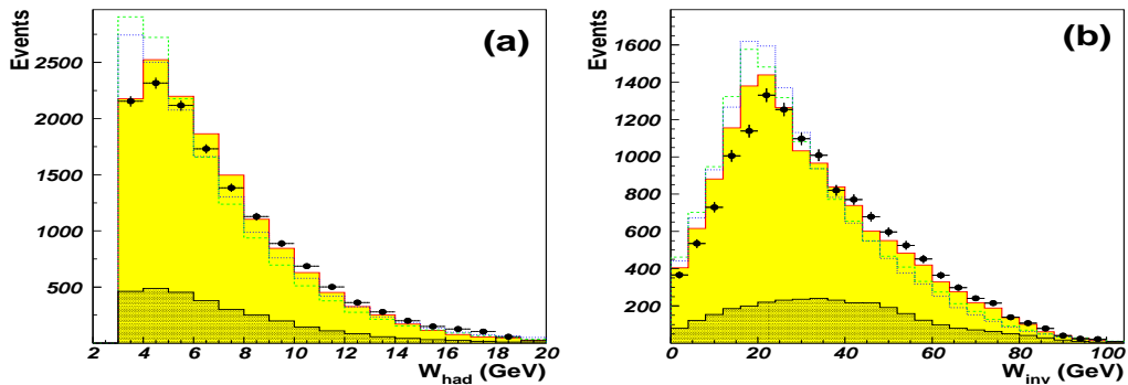
Figure 6: Comparison of single tag data and normalized Monte Carlo events: a) The invariant mass of the hadronic system, b) Reconstructed invariant mass. Points are data, the hatched area is the background, lines show Monte Carlo: solid line and shaded area is TWOGAM, the dashed line is PHOJET, and the dotted line is PYTHIA.
