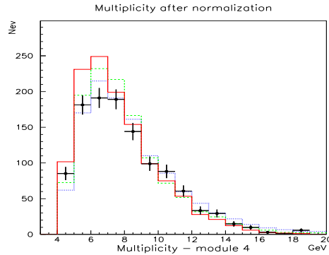
Figure 7.4: The multiplicity distribution of single tag events measured by module 4 of VSAT in year 2000 after normalization. The points are data, TWOGAM is shown as a solid line, PHOJET as a dashed line and PYTHIA as a dotted line.
