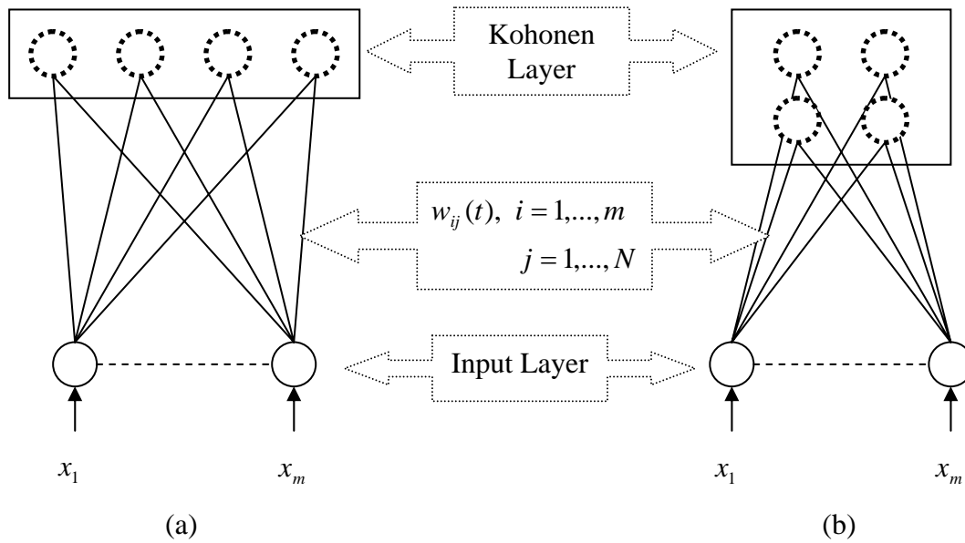
Figure 3.2. (a) A one-dimensional self-organizing map (SOM) with 4 neurons in the Kohonen layer, (b) a two-dimensional self-organizing map (SOM) with 2 \times 2 neurons in the Kohonen layer
