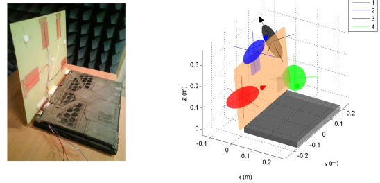
Fig. 4. Photo of the laptop computer equipped with four antennas (left) and radiation centers with current distributions axes (right).
