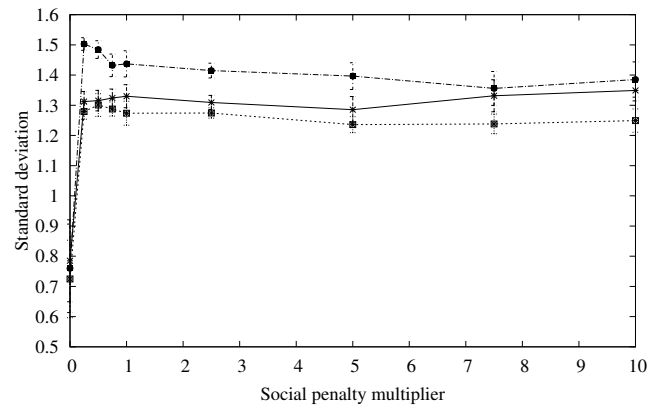
Fig. 11. Standard deviation of average vehicle speeds
