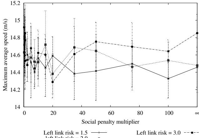
Fig. 9. Maximum average vehicle speed
