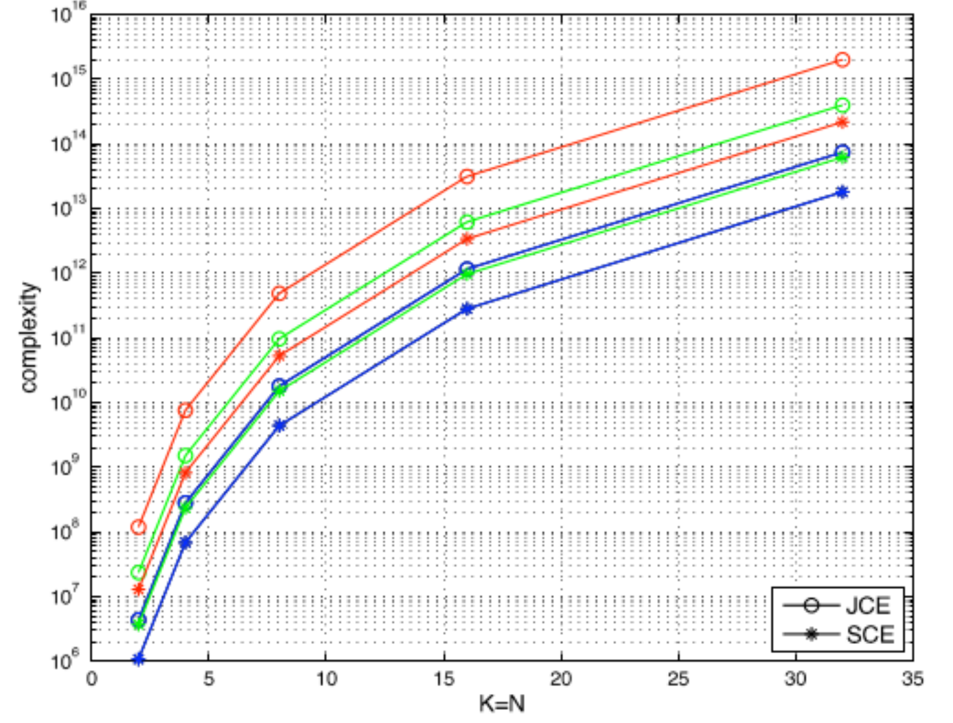
Fig. 3. Computational complexity of JCE and SCE, for M = 64 and \nu_{\max}^{(D)} = 0.05 , in the following cases: (i) S = 64, \eta_{\max}^{(d)} = 0.05 in blue; (ii) S = 80, \eta_{\max}^{(d)} = 0.07 in green; (iii) S = 96, \eta_{\max}^{(d)} = 0.1 in red.
