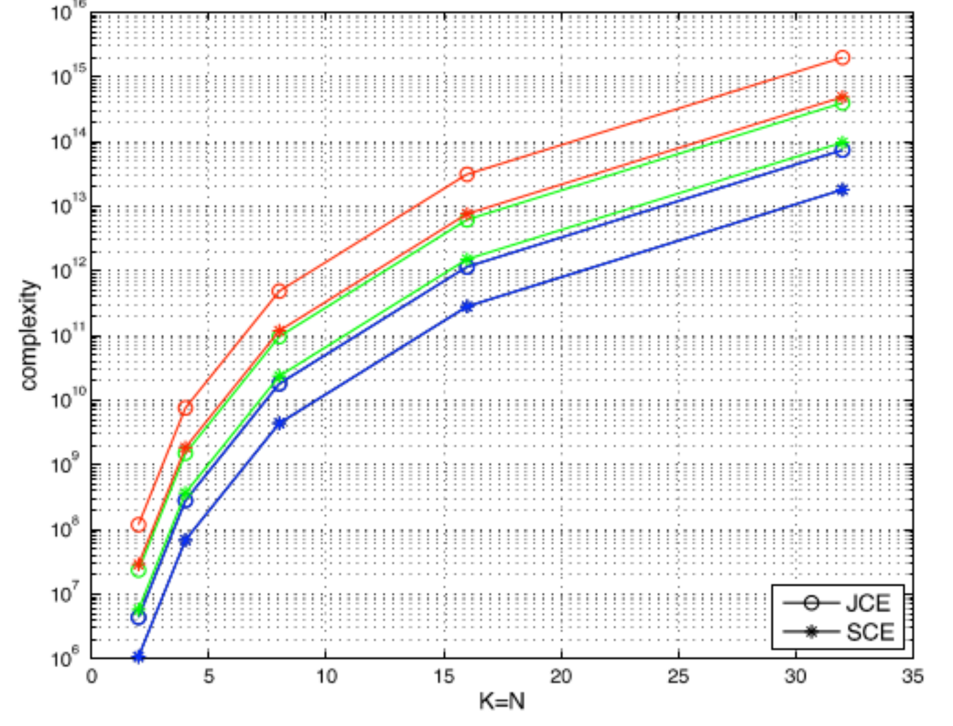
Fig. 2. Computational complexity of JCE and SCE, for S = 64 and \nu_{\max}^{(D)} = 0.05 , in the following cases: (i) M = 64, \eta_{\max}^{(d)} = 0.05 in blue; (ii) M = 80, \eta_{\max}^{(d)} = 0.07 in green; (iii) M = 96, \eta_{\max}^{(d)} = 0.1 in red.
