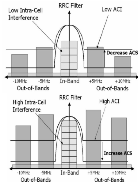
Figure 2. Spectrum analysis of operational concept of reconfigurable filter
