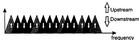
Fig. 1. The Zipper principle of capacity division.
