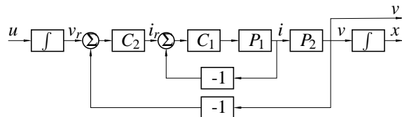
Figure 1. Cascaded control structure for the cart control.
