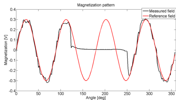
Figure 8: Magnetization, showing the reference pattern and the measured pattern. No workpiece is used at the position angles of 140-240 degrees, hence measured values are zero here.
