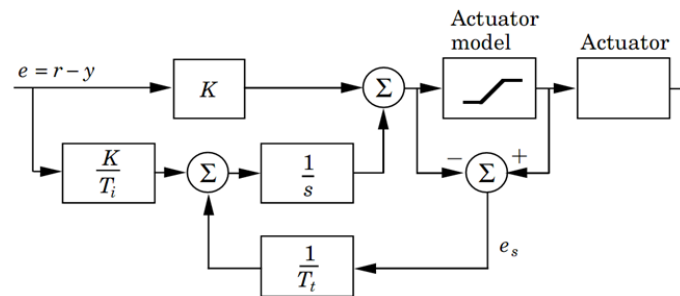
Figure 5: A PI-controller using an implementation of a classical anti-windup type. [8]
