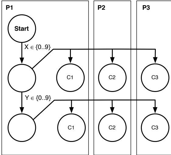
Figure 3: Parallel consistency in constraint programming.
