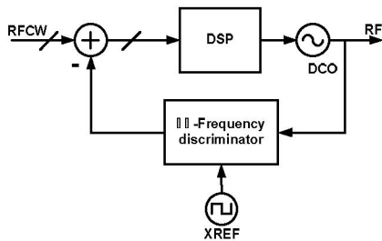
Figure 2. An All-Digital \Sigma\Delta FD-based Frequency Synthesizer
