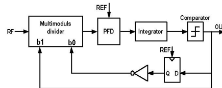
Figure 4. Single loop second order \Sigma\Delta Frequency Discriminator [5]
