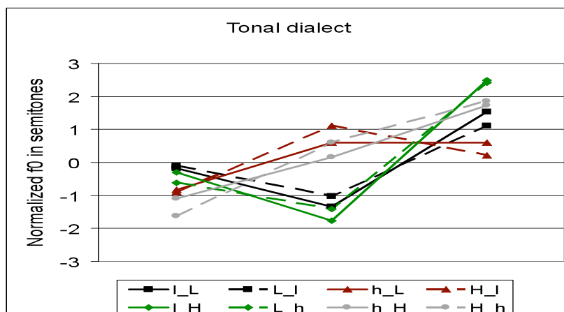
Figure 3. Normalised F0 measurement points for the tonal dialect. Measurement points are F0 maxima in the three last words (copula + [noun+adjective]) of sentences of type “This is [noun+adjective]”. Lexical tone and focal status are indicated for the last two words. l=low lexical tone, h=high tone, L/H=focus.
