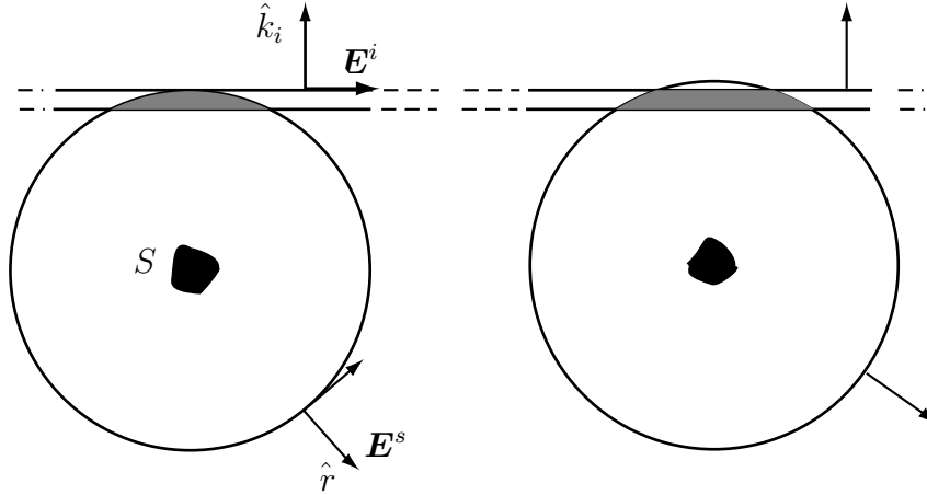
Figure 5: The scattering object, the incident wave and the scattered wave. The figure to the right shows a case when the wave speed inside the scattering object is larger than for the surrounding medium.
