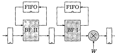
Figure 1: Part of the FFT processor pipeline. The butterfly processors are named "BF I" and "BF II". Shaded boxes are combinatorial logic.
