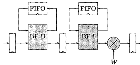
Figure 1: Part of the FFT processor pipeline. The butterfly processors are named "BF I" and "BF II". Shaded boxes are combinational logic.
