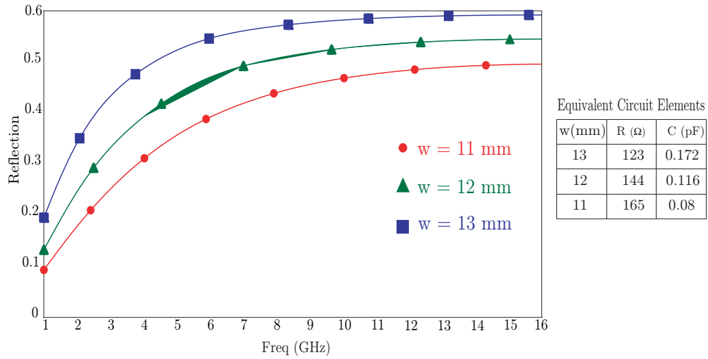
Figure 5: Frequency response (reflection coefficient) and equivalent circuit element values for a typical square patch, at normal incidence. ( a = 14 mm, R_s = 100 \Omega/\text{Sq} )
