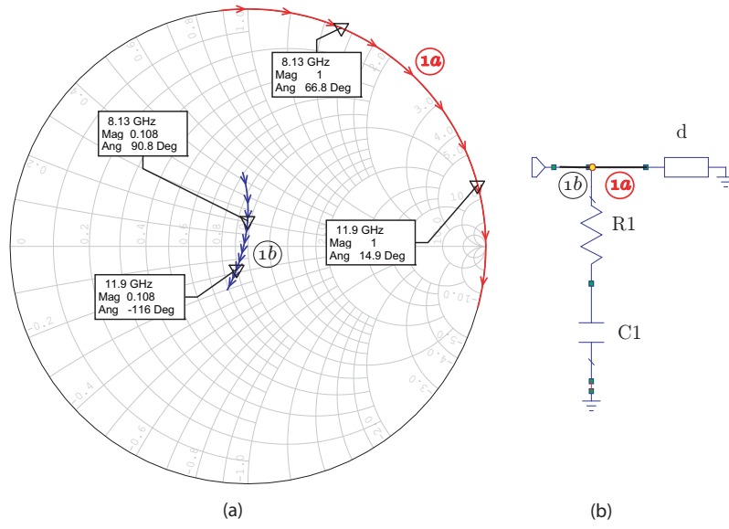
Figure 8: The equivalent circuit model of the thin wideband capacitive circuit absorber. (a) The reflection coefficient at points 1a and 1b. (b) The schematic of the single layer capacitive circuit absorber.
