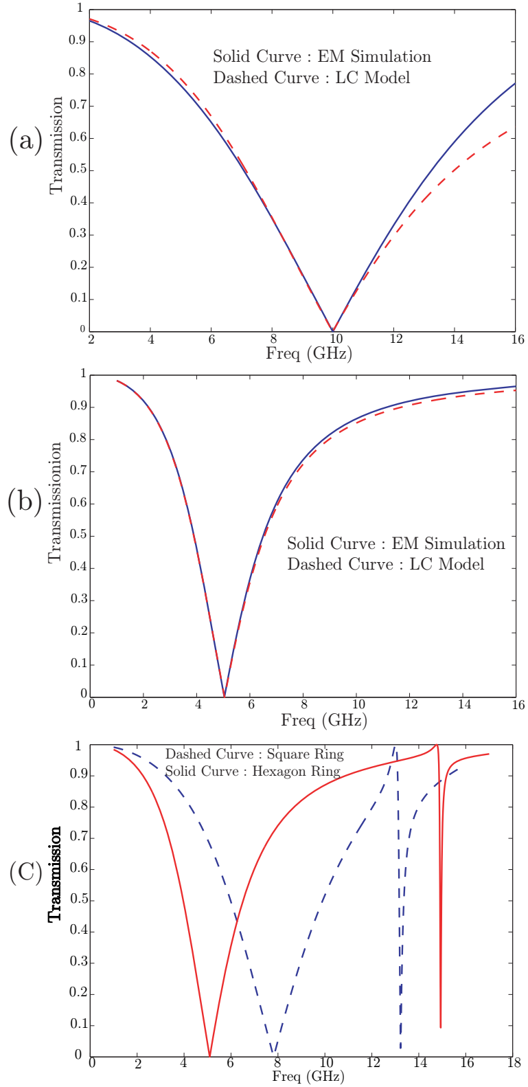
Figure 6: The frequency response (transmission coefficient) of a square and hexagon ring indicating the effect of harmonics on the RLC model bandwidth. (a) Normal incidence, Square ring (b) Normal incidence, Hexagon ring (c) Oblique angle of incidence = 15^\circ . (periodicity in x-direction 1.4 cm)
