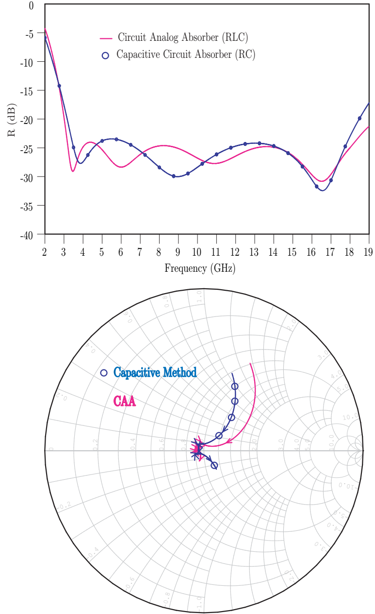
Figure 7: The frequency response of a three layered circuit analog absorber compared with a three layered capacitive circuit method. (Circuit Model, Operating band 3–18 GHz, return loss = 25 dB)
