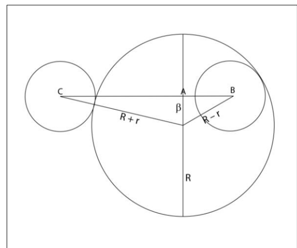
Figure 4: Eclipse geometry.
