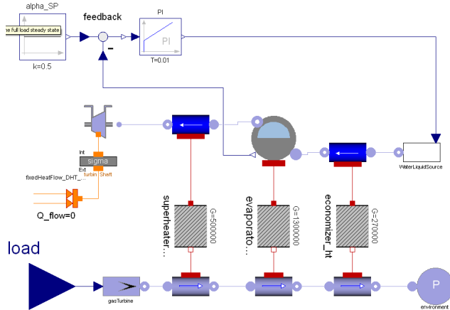
Figure 5: Diagram of the combined-cycle plant model.
