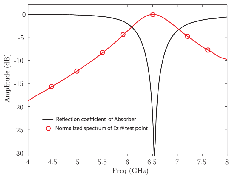
Figure 6: Frequency response of the absorber (solid curve) and the normalized spectrum of the E_z component at test point (circled curve).
