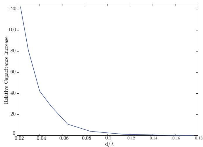
Figure 3: The relative capacitance increase \left(\frac{C_{\text{adj}} - C_{\text{grating}}}{C_{\text{grating}}}\right) as a function of thickness to wavelength ratio. ( a = 40 mm, w = 27 mm, \epsilon_r = 1.2 )
