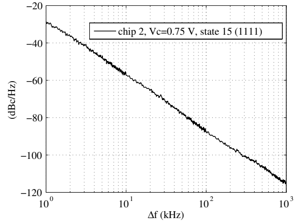
Fig. 8. Phase Noise, state 15 (1111) & V_c=0.75 V, for chip 2
