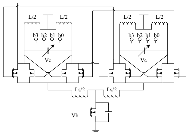
Fig. 1. QVCO Schematic
