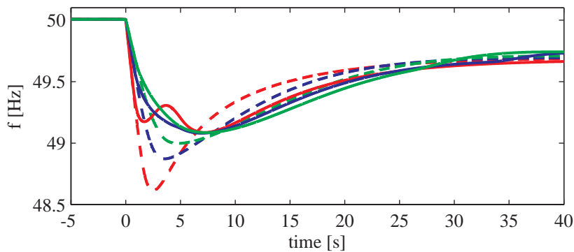
Figure 7.18 30 000 MW load. Loss of 1400 MW generation with uncontrolled (dashed) and controlled wind power (solid). S_n H=50 GWs (red), 75 GWs (blue) and 100 GWs (green). P_{inc}=10\% , proportional to \Delta f .
