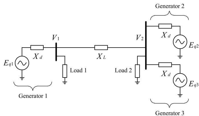
Figure 2.1 Simple power system model.
