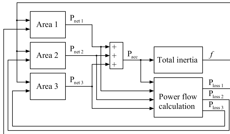
Figure 3.4 Power system model with 3 areas.
