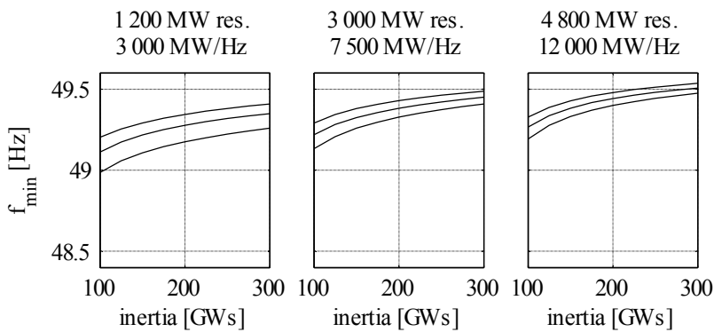
Figure 5.5 f_{\min} due to loss of 1 400 MW production with different reserve and load. From top 60 000, 45 000 and 30 000 MW load. Predisturbance frequency 50.0 Hz.
