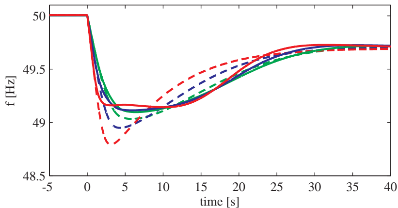
Figure 7.12 30 000 MW load, loss of 1 400 MW thermal production. Wind power without control (dashed). Wind power with \Delta f -controller (solid). t_{inc}=5 s t_{dec}=20 s. 10% (green), 20% (blue) and 30% (red) wind power. P_{ref}=P_{order}+P_{inc}
