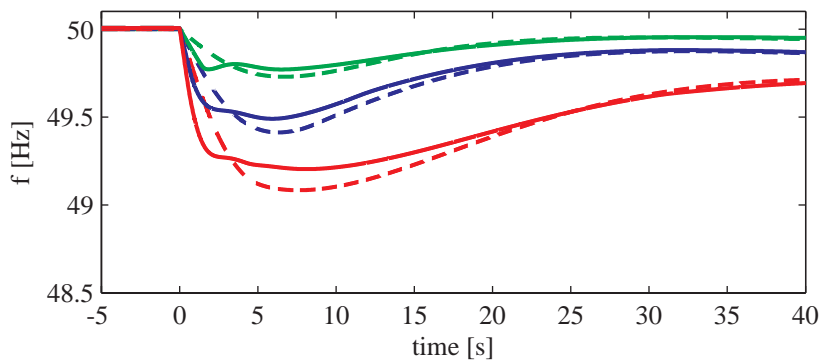
Figure 6.19 df/dt -controller with 0.05 Hz filter on measured frequency. Loss of 400 MW (green), 900 MW (blue) and 1 400 MW (red) generation. Without wind power (dashed), with controlled wind power (solid).
