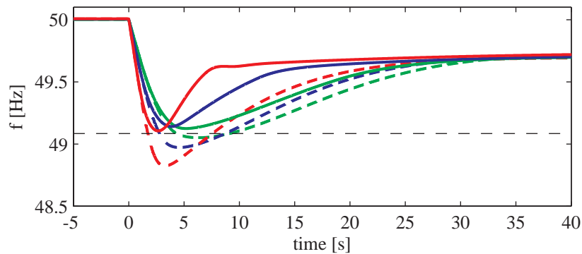
Figure 7.21 30 000 MW load. Loss of 1400 MW generation. Curtailed wind power with droop control. P_{inc} = 4\% linearly increased between 49.9 and 49.5 Hz. Uncontrolled (dashed) and controlled wind power (solid). 15 000 MW installed wind power producing 0.8 pu (red), 0.5 pu (blue) and 0.2 pu (green). Black dashed line indicates lowest frequency without wind power.
