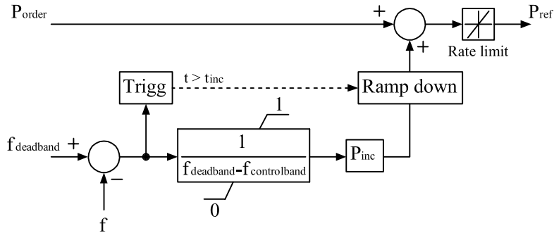
Figure 7.9 \Delta f -controller.
