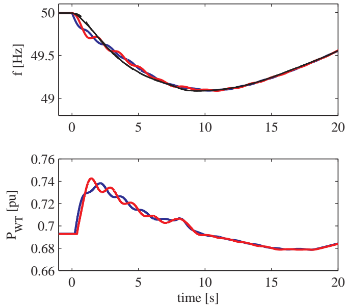
Figure 6.14 High wind power, df/dt -controller with estimated average frequency. Top: frequency at G2 (blue) and G3 (red). Estimated frequency at wind turbine bus bars (black). Bottom: power from wind turbine connected at bus 1 (blue) and bus 4 (red).
