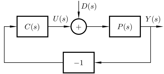
Fig. 1. Closed-loop system with process P(s) , controller C(s) , output Y(s) , and load disturbance D(s) .
