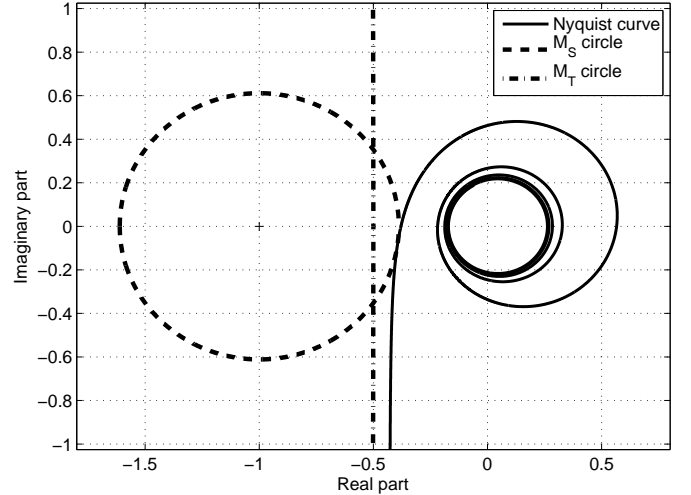
Fig. 10. Nyquist curve for P(s) = K/(sT+1)e^{-sL} with T_d = 5T = 5 and L = 9 and corresponding circles for M_S = 1.64 and M_T = 1 .
