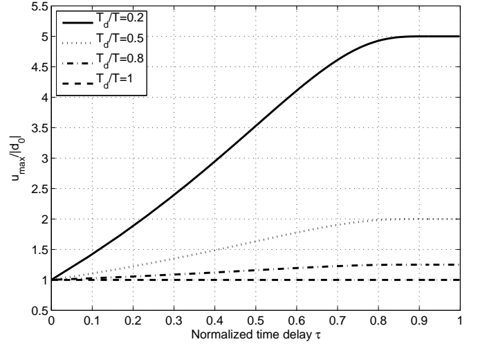
Fig. 4. Maximum magnitude u_{\max} of control signal as function of normalized time delay \tau .
