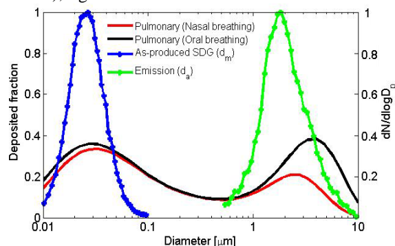
Figure 2. Two pulmonary deposition curves (MPPD) shown together with typical particle number size distributions (normalized) of as-produced particles and emitted particles during maintenance of the generators.
