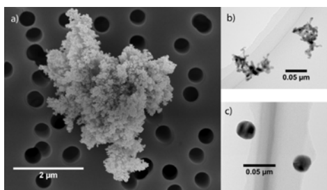
Figure 1. a) Typical emitted agglomerate with nanostructures related to sintered particles. b) Aggregates formed by the SDG. c) Sintered particles
