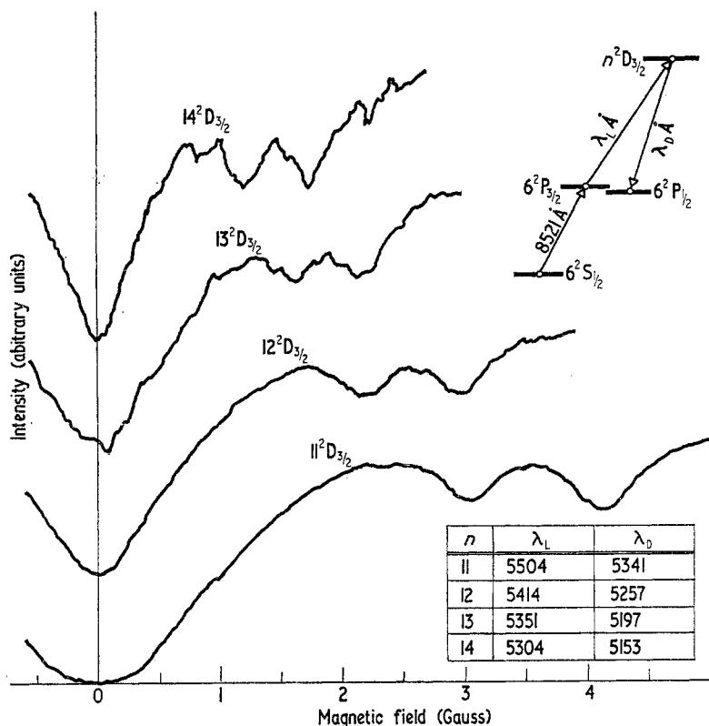
Figure 1. Level crossing signals for the 11, 12, 13, and 14 ^2D_{3/2} states in ^{133}\text{Cs} . The sampling time for each of the curves is 0.5–1 h.
